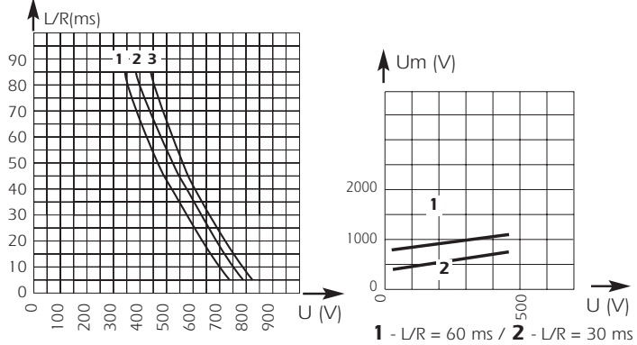
Above: Curves indicate permissible value of time constant L/R as a function of DC working voltage. 1 - I_N from 80 to 110 A / 2 - I_N from 25 to 63 A 3 - I_N from 8 to 12 A
